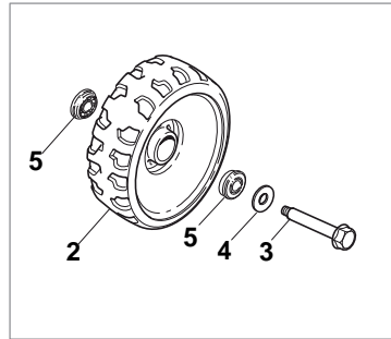
BALL BEARING Version - Ø 165
